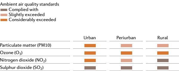
G10 Exceedance of ambient air quality standards established by the Ordinance on Air Pollution Control (LRV), 2010
