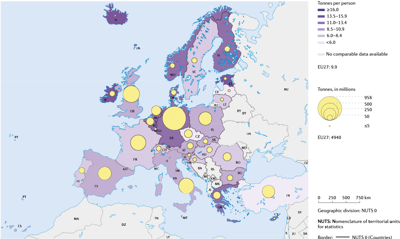
MIII.2 Greenhouse gas emissions in CO 2 equivalents, 2008
