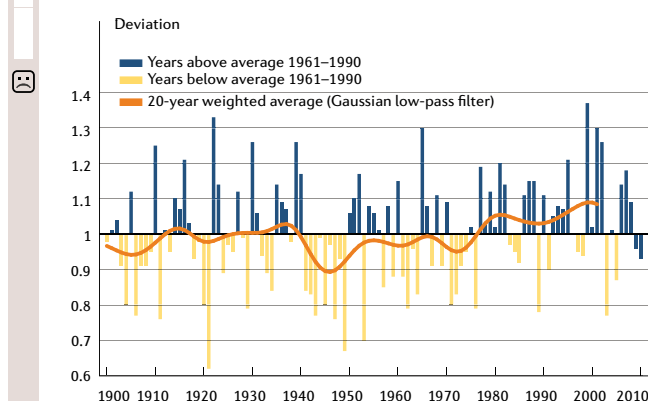
G8.1 Mean annual precipitation in Switzerland Deviation from the mean 1961–1990
